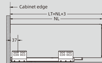
16mm panel
