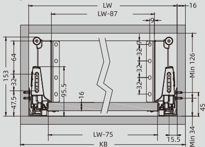
16mm panel
