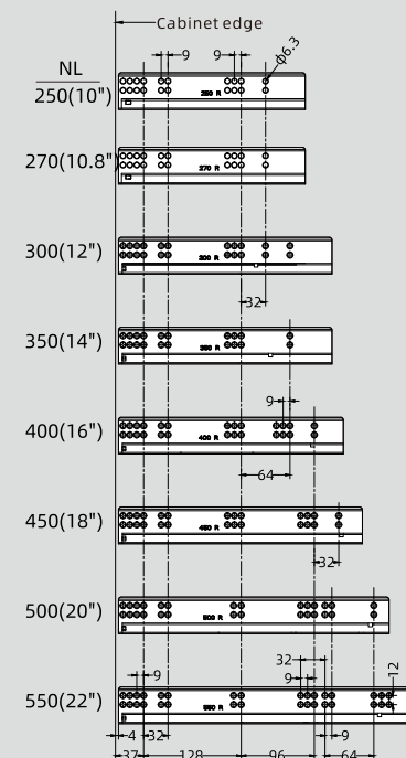
16mm panel
