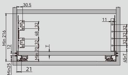
16mm panel
