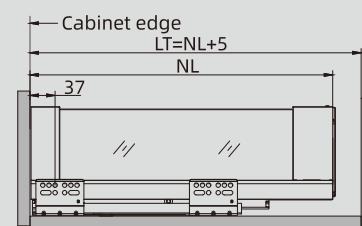
18mm panel
