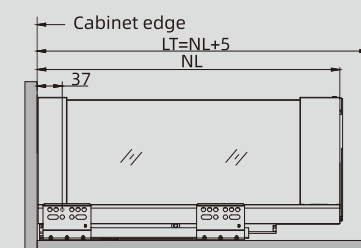
18mm panel
