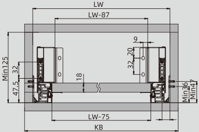
18mm panel
