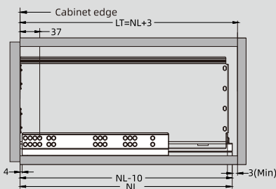
16mm panel
