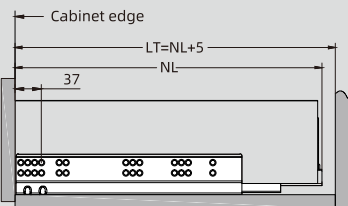
16mm panel
