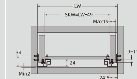
18mm panel
