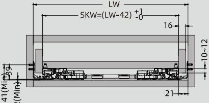
16mm panel
