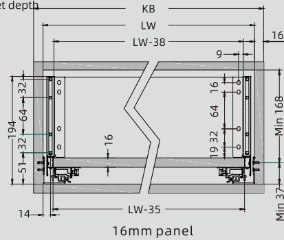
16mm panel
