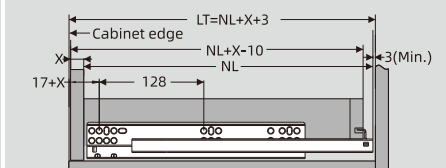
16/18mm panel
