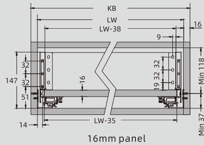
16mm panel
