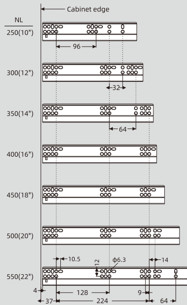
16/18mm panel
