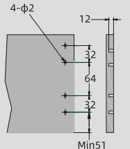
16mm panel
