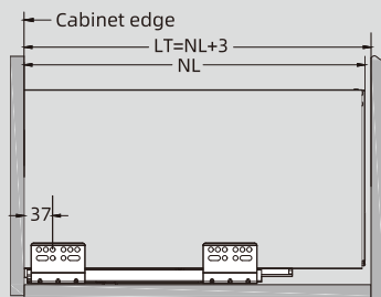
16mm panel
