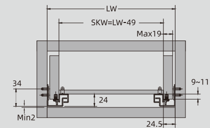
18mm panel
