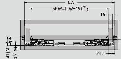
18mm panel
