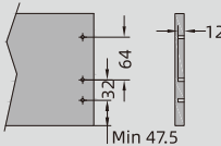
16mm panel
