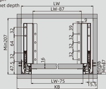
16mm panel
