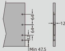
16mm panel
