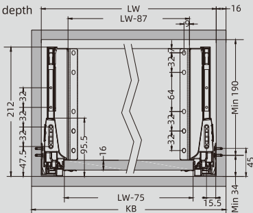
16mm panel
