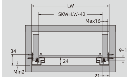
16mm panel
