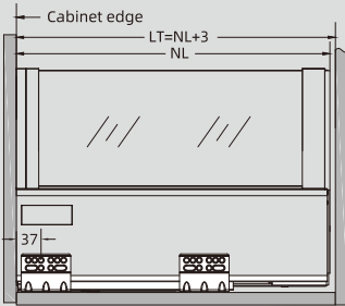
16mm panel
