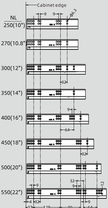
16mm panel
