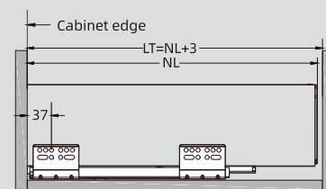
16mm panel
