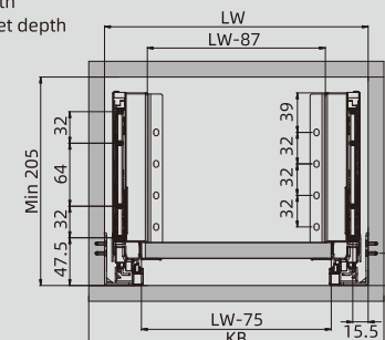
18mm panel
