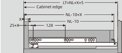
16/18mm panel
