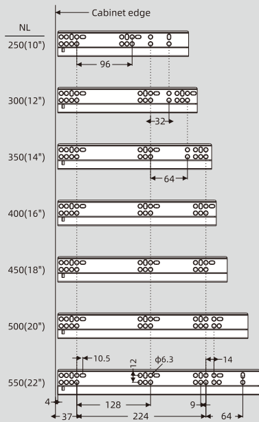
16/18mm panel
