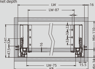
18mm panel
