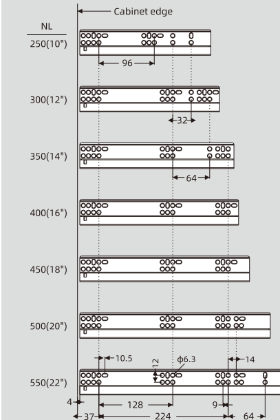
16/18mm panel
