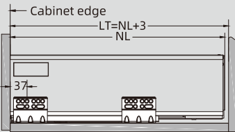
16mm panel
