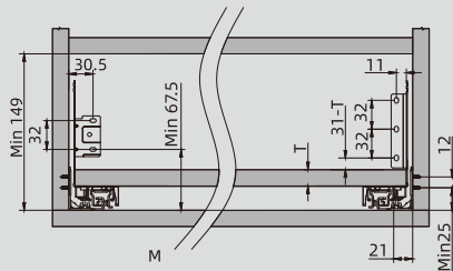
16mm panel
