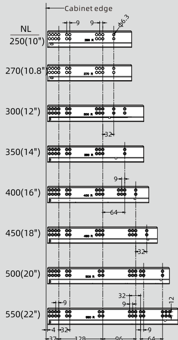
16mm panel
