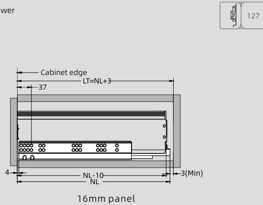
16mm panel
