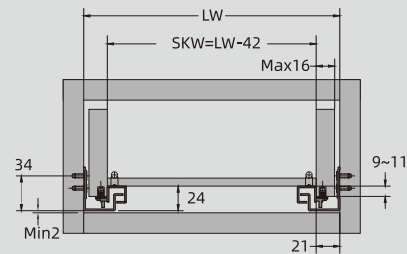
16mm panel
