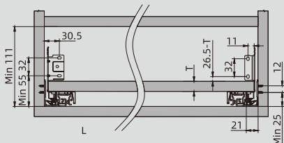
16mm panel
