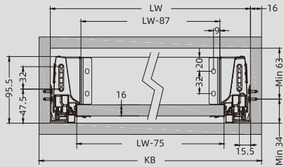
16mm panel
