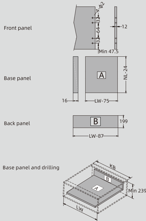
16mm panel
