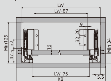
16mm panel
