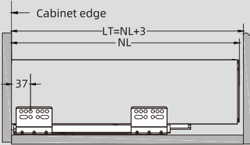
18mm panel
