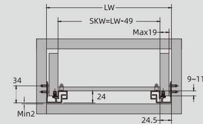
18mm panel
