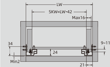
16mm panel
